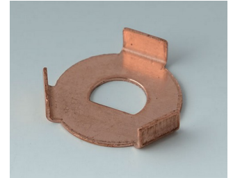
A6600064 Protection anti-rotation 6/4,6
