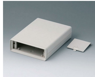
A9413638 BOITIER COQUILLES V 190, Vers. V ABS (UL 94 HB) gris blanc RAL 9002 138x190x45mm
