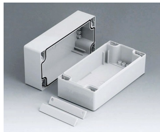
C2108162 ROBUST-BOX 80 BREIT, Ausf. II PC (UL 94 HB) lichtgrau RAL 7035 160x80x80mm IP 66
