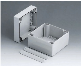
C2112121 ROBUST-BOX 120 BREIT, Ausf. I ABS (UL 94 HB) lichtgrau RAL 7035 120x120x90mm IP 66
