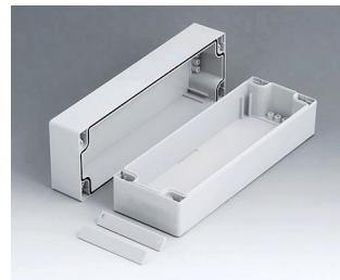
C2108241 ROBUST-BOX 80 BREIT, Ausf. I ABS (UL 94 HB) lichtgrau RAL 7035 240x80x80mm IP 66
