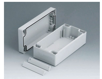
C2008162 ROBUST-BOX 80 BREIT, Ausf. II PC (UL 94 HB) lichtgrau RAL 7035 160x80x60mm IP 66
